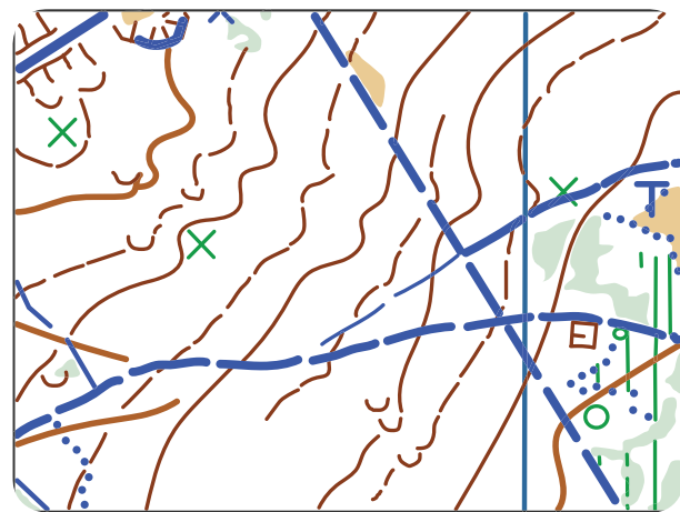
Figure 10.3 Form lines
