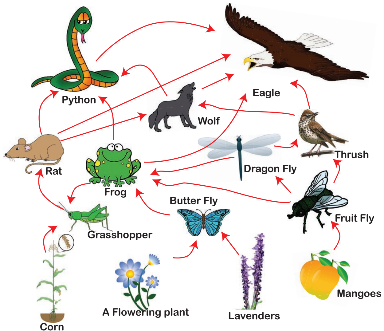
Figure 7.4 Food web
