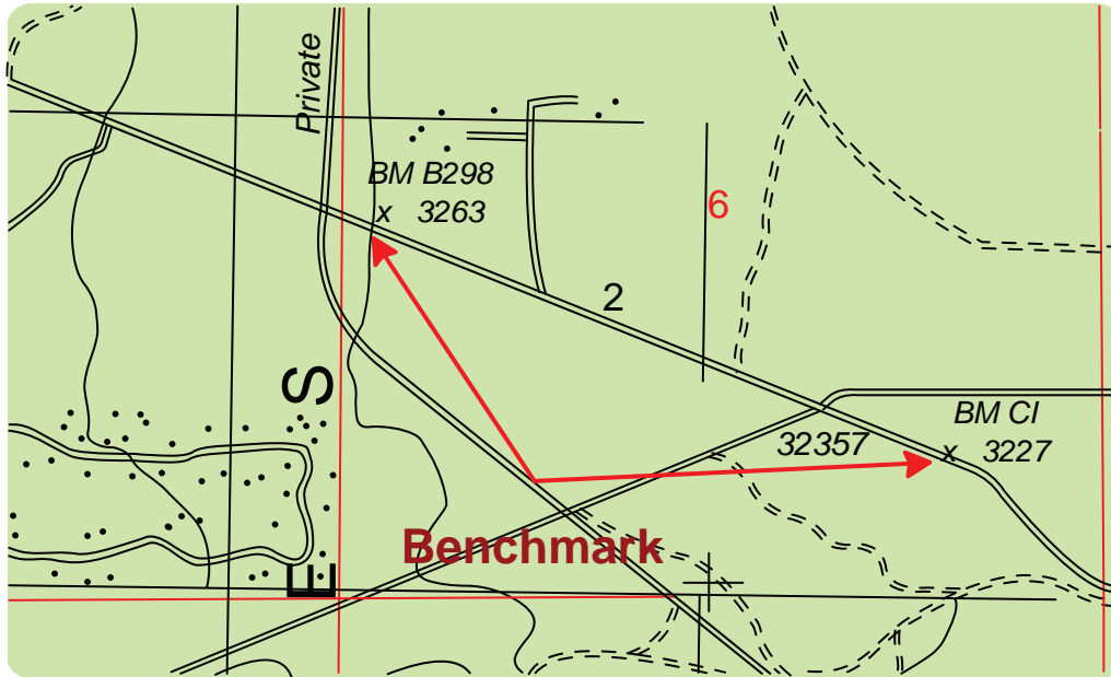
Figure 10.5 Benchmark
