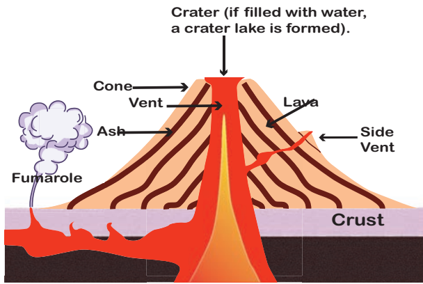
Figure 3.25 Volcano
