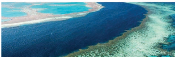
Barrier Reef
