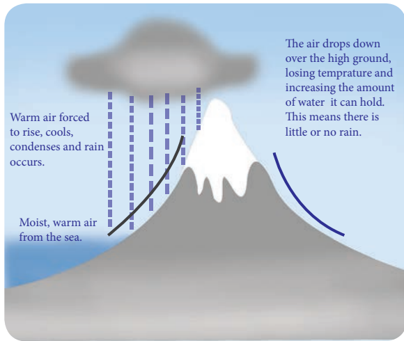
Figure 6.26 Orographic Rainfall
