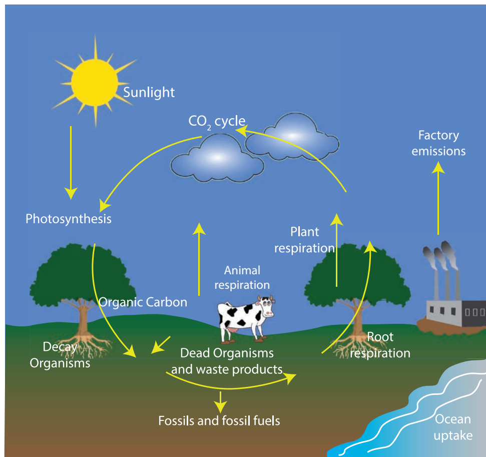
Figure 7.6 Carbon Cycle
