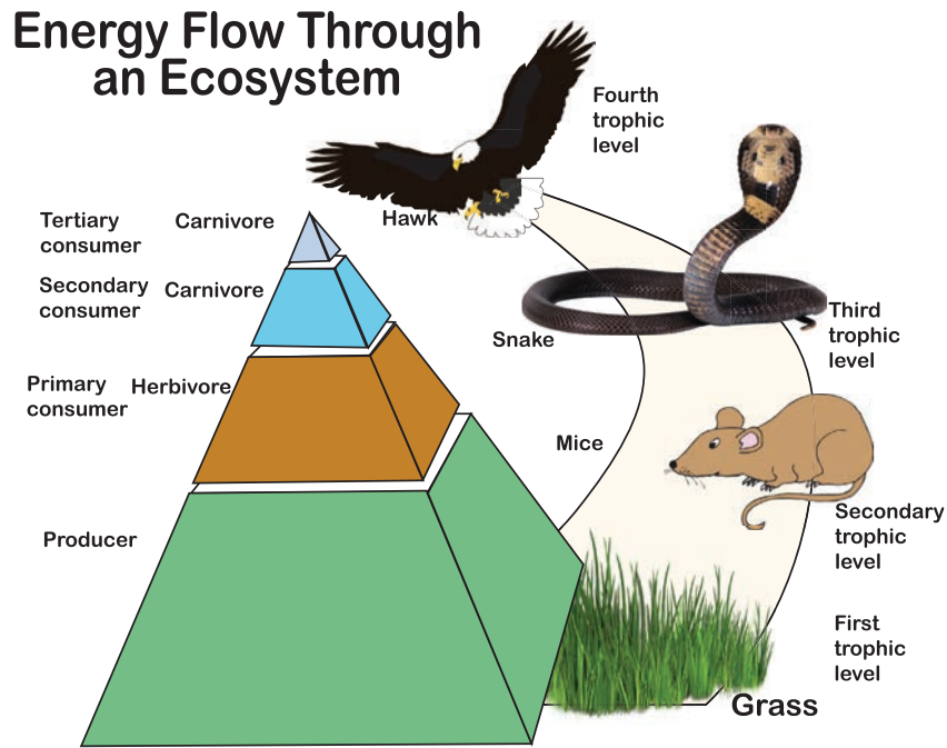
Figure 7.5 Energy Pyramid
