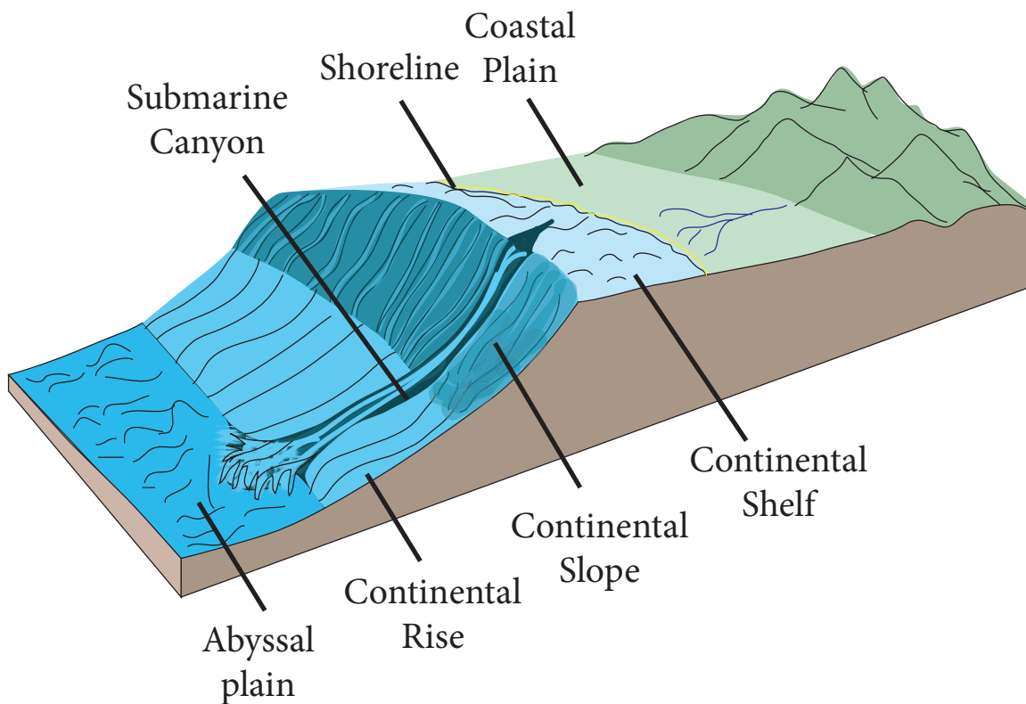
Figure 5.8 Ocean relief
