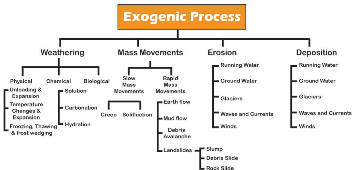
Figure 4.1 Exogenic processes
