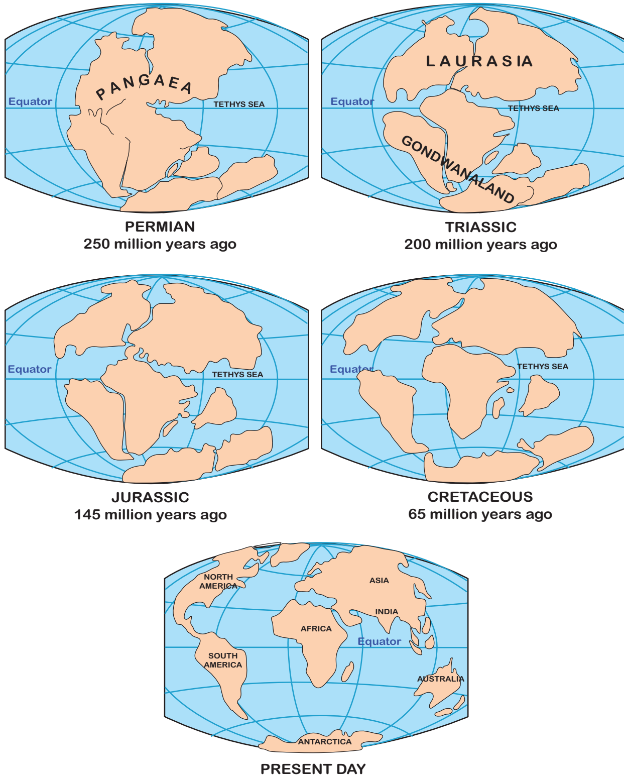
Figure 3.5 Continental Drift
