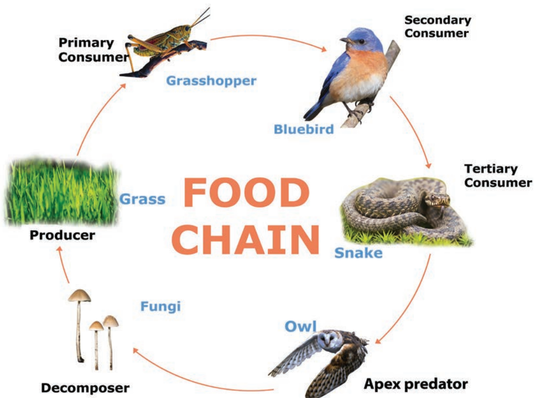
Figure 7.3 Food Chain
