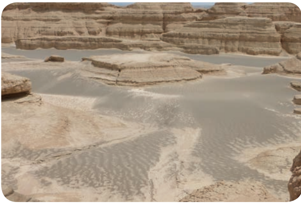
Figure 4.25 Zeugen
