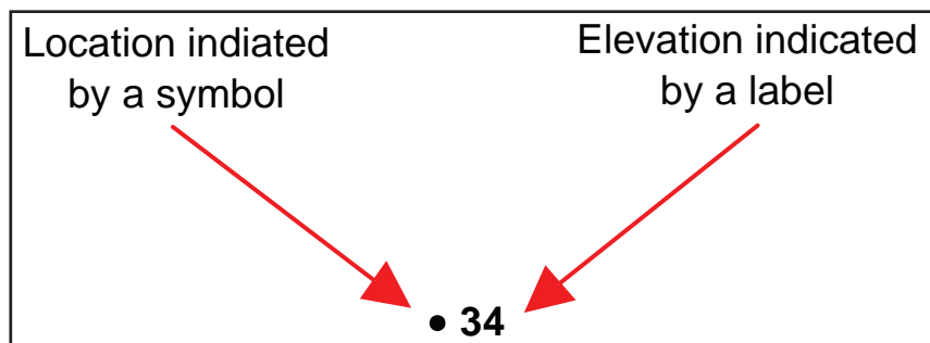
Figure 10.2 Contours
