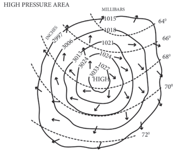
Figure 6.36 Anticyclone
