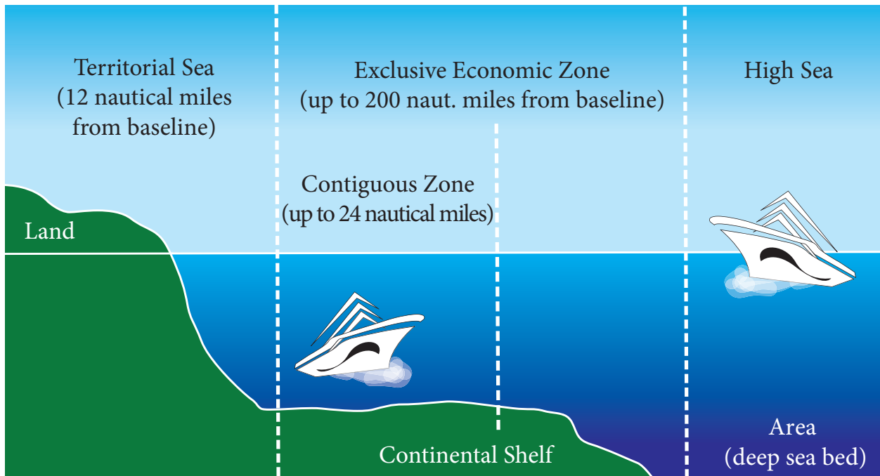
Figure 5.5 Maritime Zones
