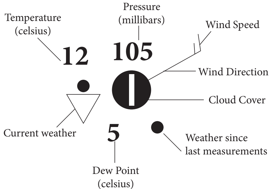
Figure 12.2 Station model
