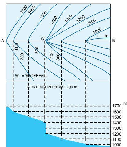
Figure 10.15 Waterfall
