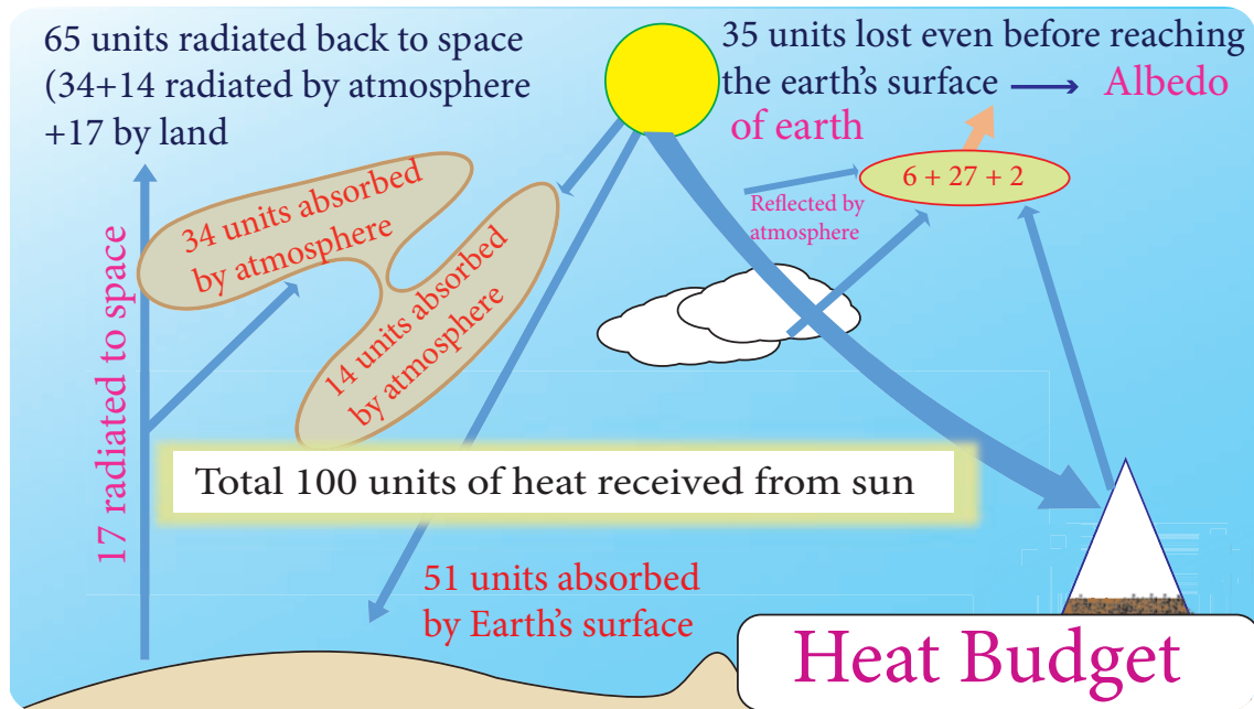
Figure 6.6 Heat Budget
