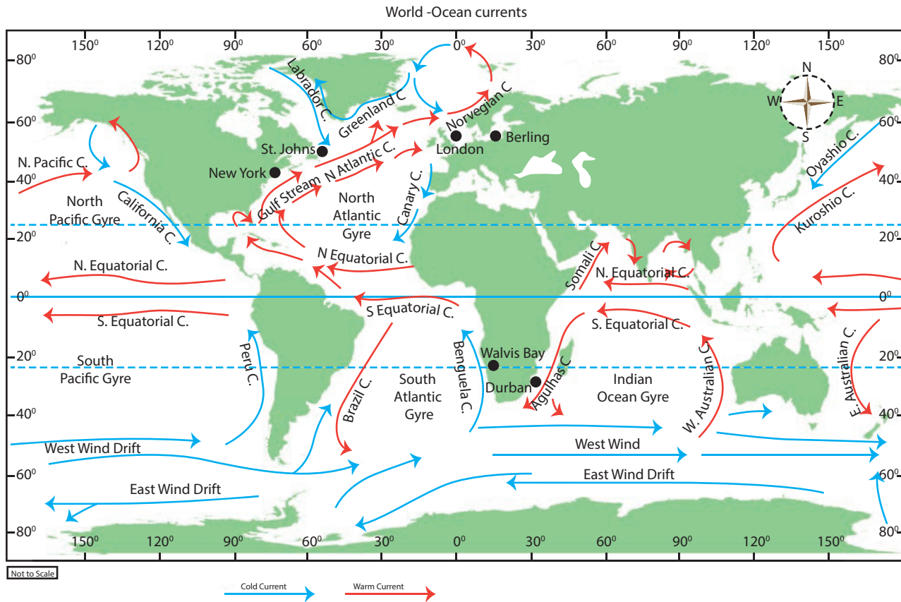
Figure 5.18 World-Ocean currents
