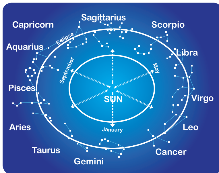
Figure 2.3 Constellation
