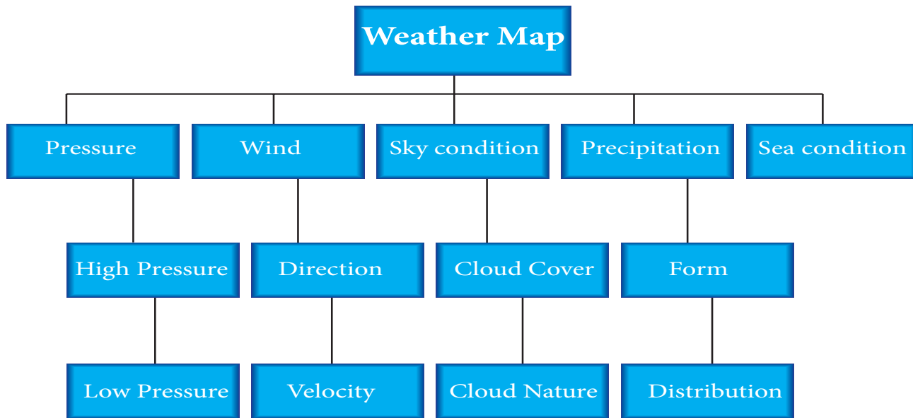
Figure 12.3 Wether Map
