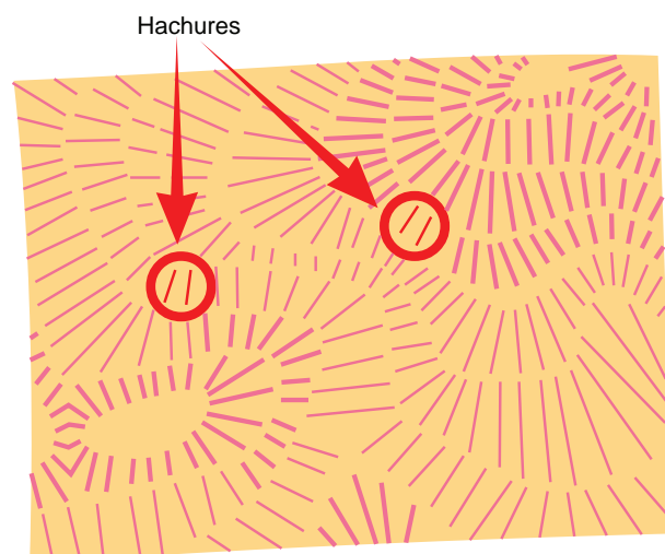
Figure 10.1 Hachures
