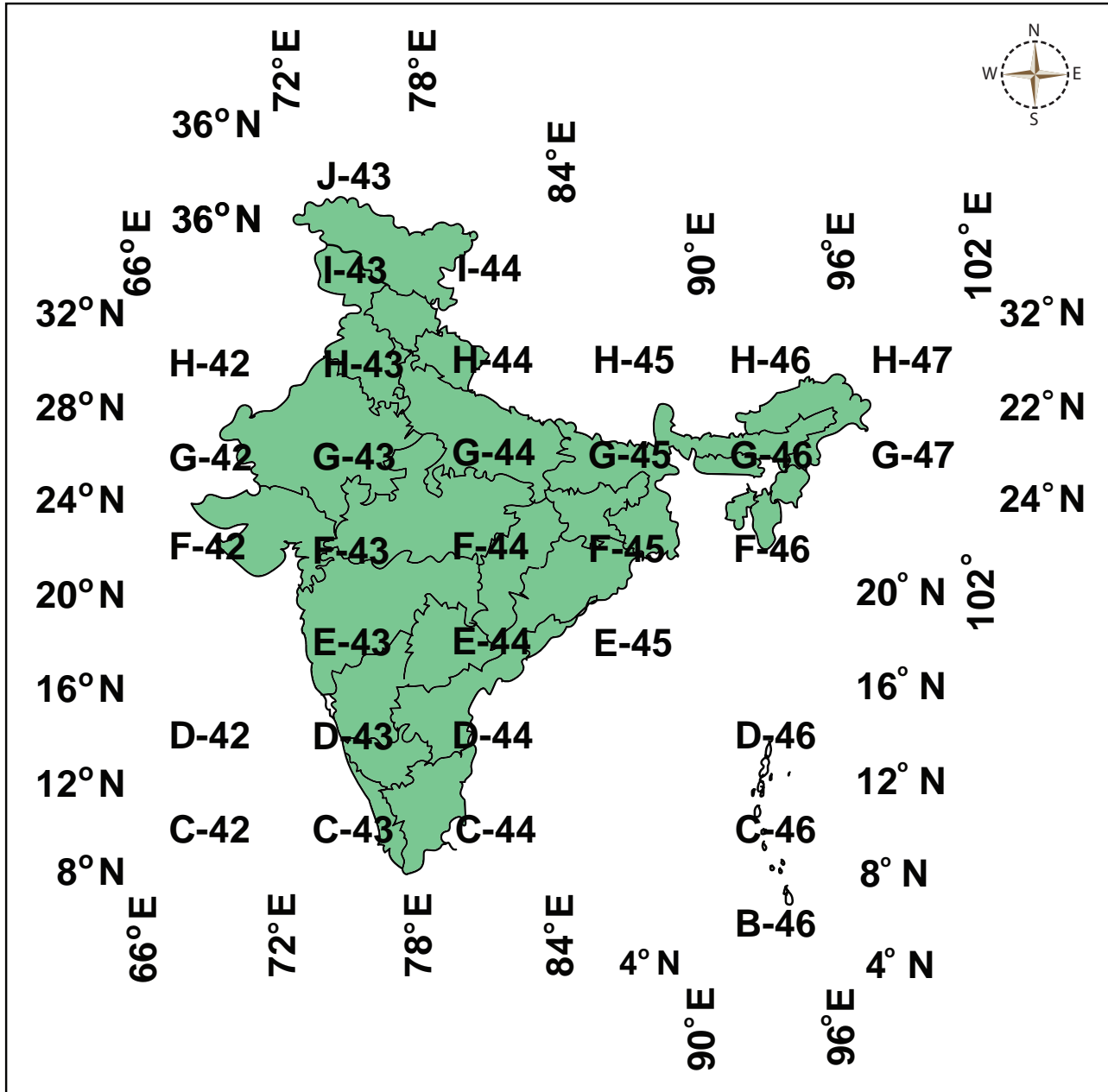
Figure 11.3 Index System
