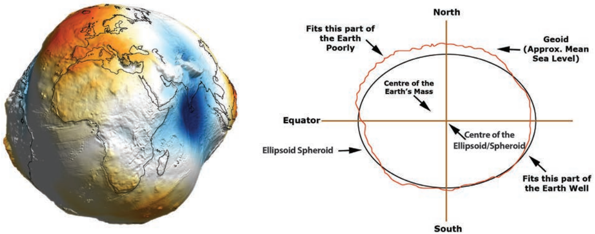
Figure 2.9 Geoid : Shape of the earth
