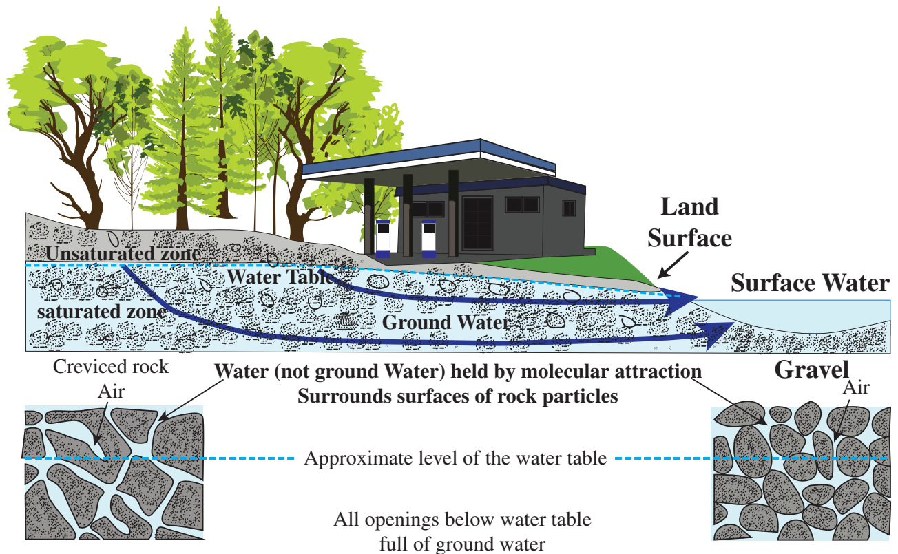
Figure 5.1 Ground water
