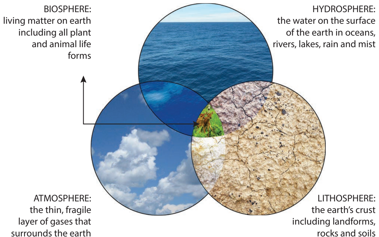
Figure 7.1 Biosphere
