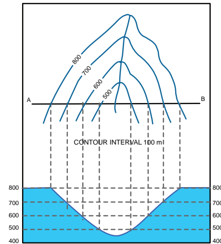
Figure 10.17 V-Shaped valley
