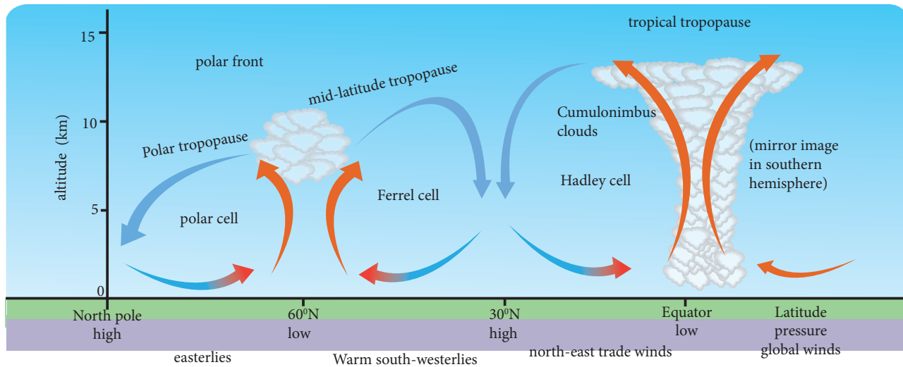
Figure 6.14 Meridional circulation
