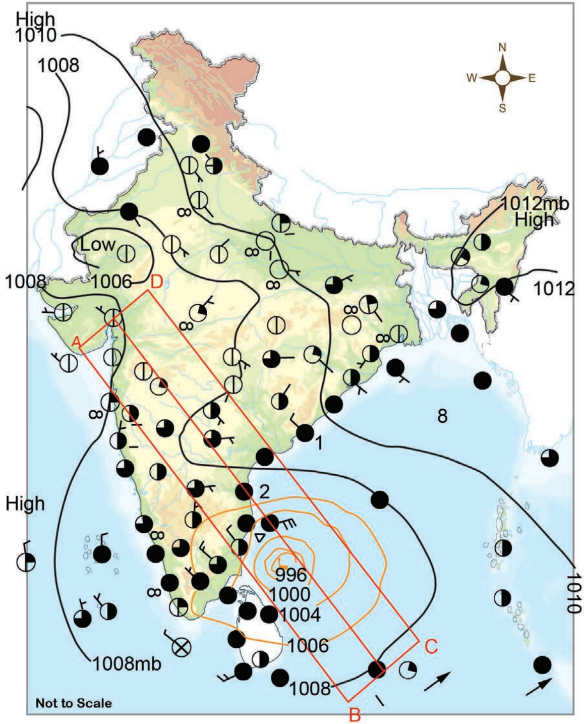
WEATHER MAP
