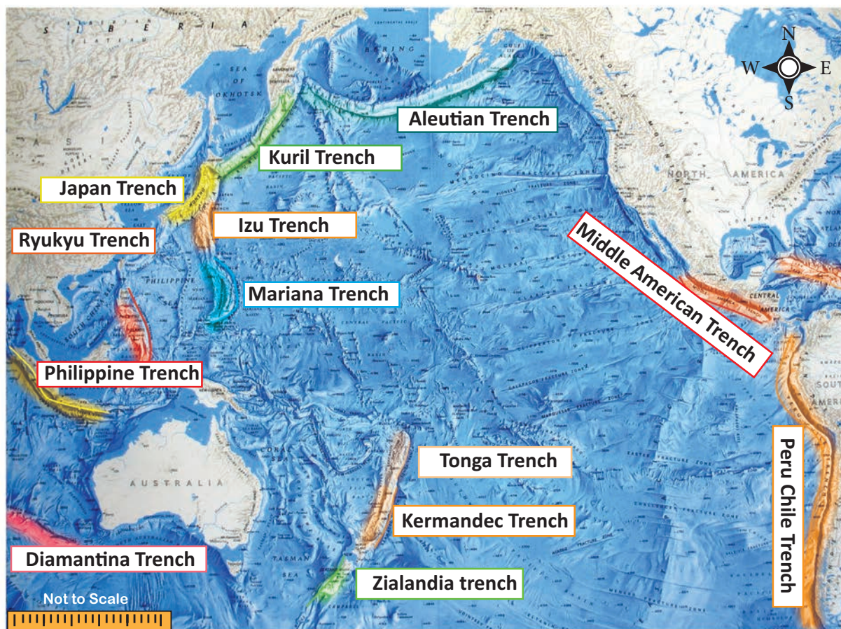
Figure 5.9a Bottom relief of Pacific Ocean
