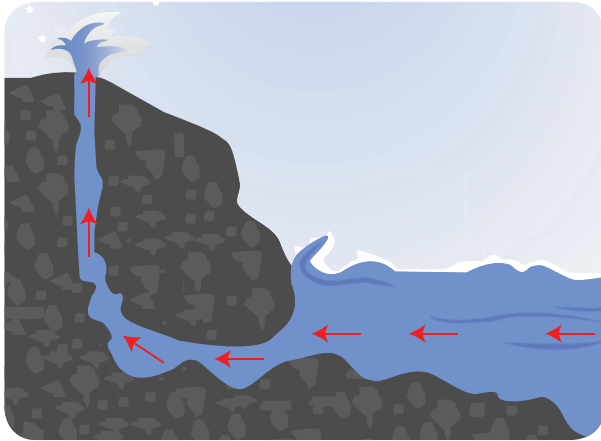
Figure 4.29 Blow hole
