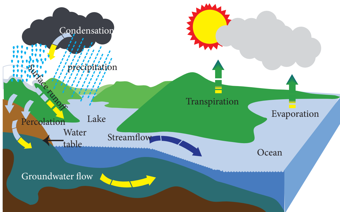
Figure 6.23 Hydrological cycle
