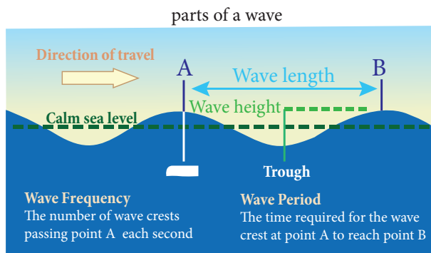
Figure 5.16 Parts of a wave
