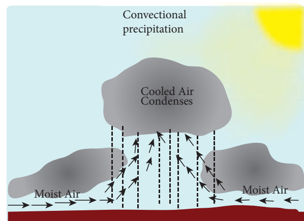
Figure 6.25 Convective rainfall
