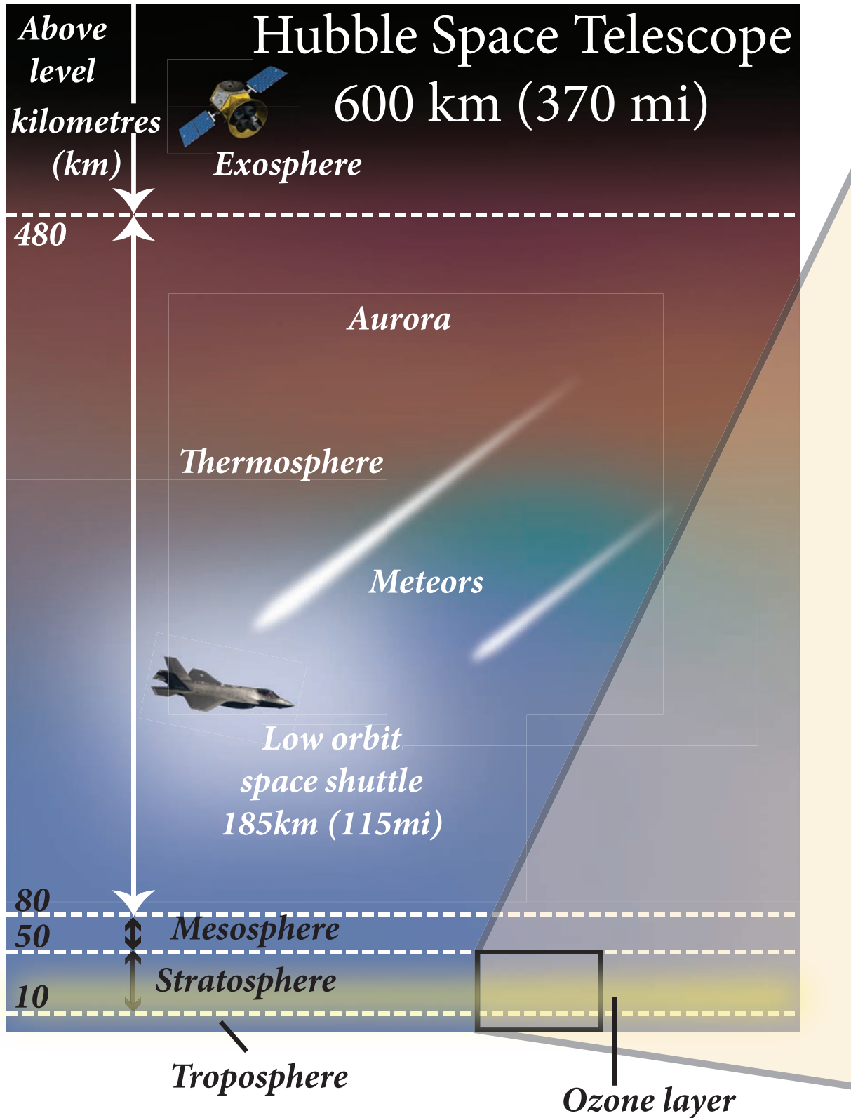
Figure 6.4 Thermosphere
