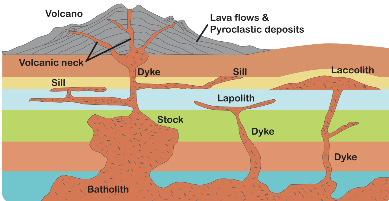
Figure 3.26 Intrusive Volcanic structure
