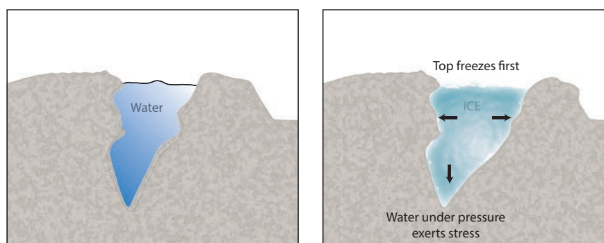
Figure 4.3 Frost Wedging
