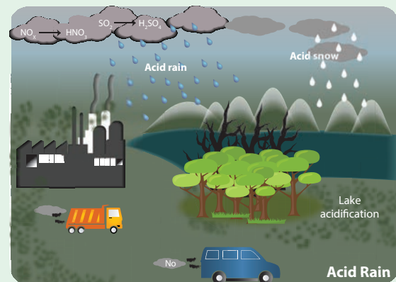
Figure 6.27 Acid rain
