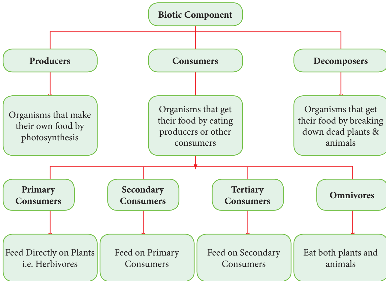
Figure 7.2 Biotic Components
