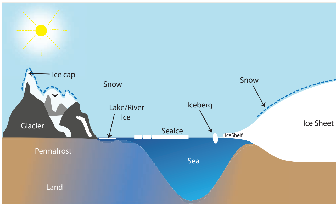
Figure 5.2 Cryosphere
