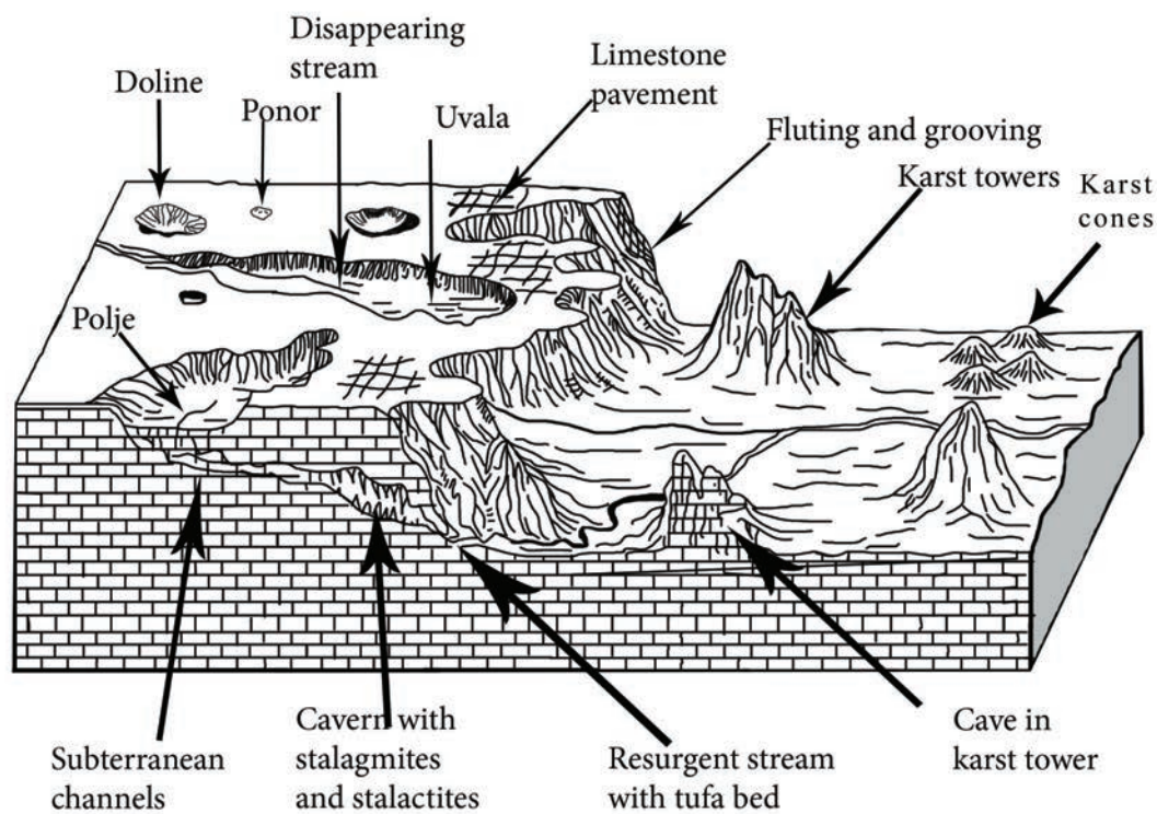
Figure 4.20 Karst features
