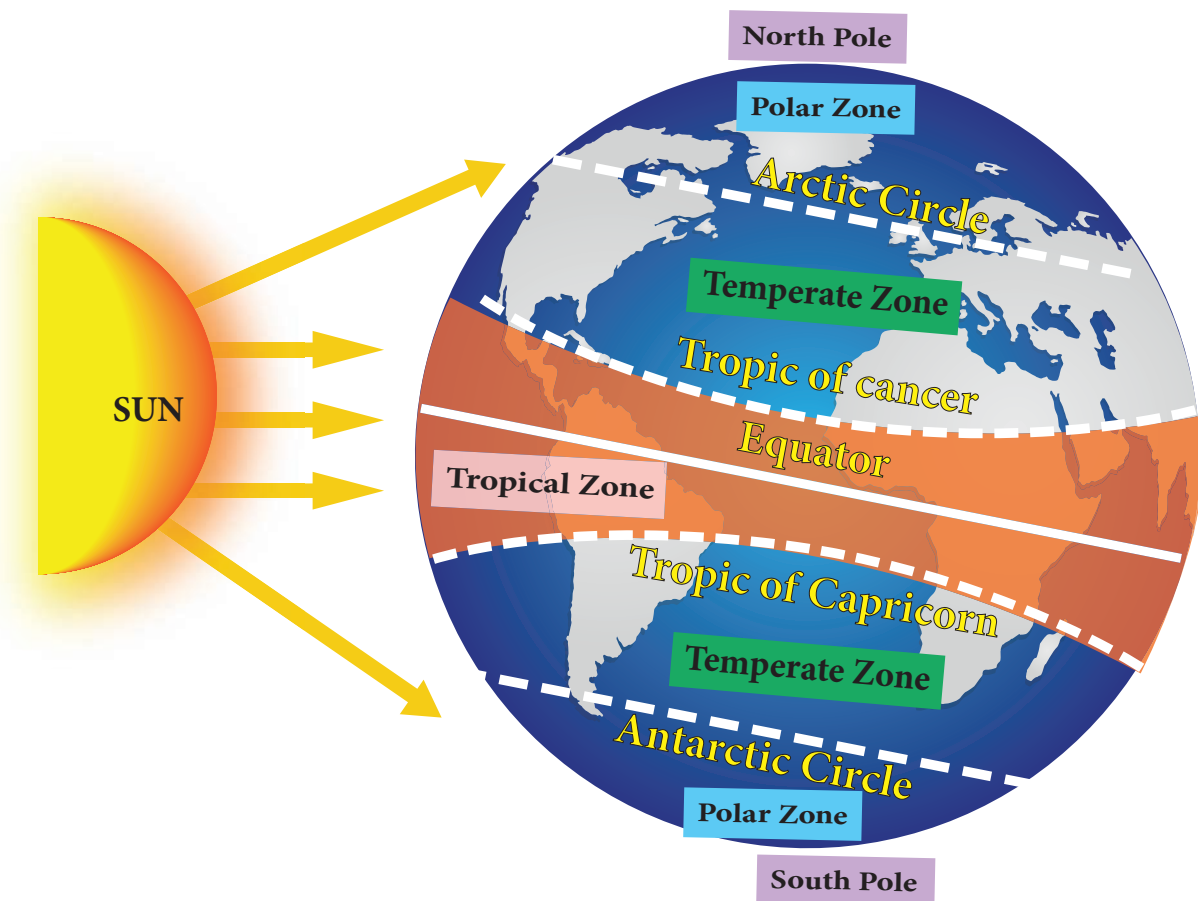
Figure 6.8 Heat Zones
