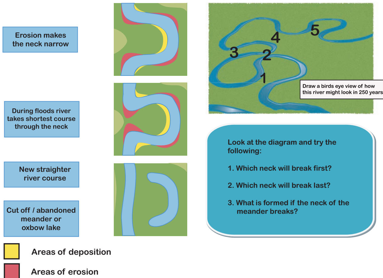
Figure 4.14 Meander
