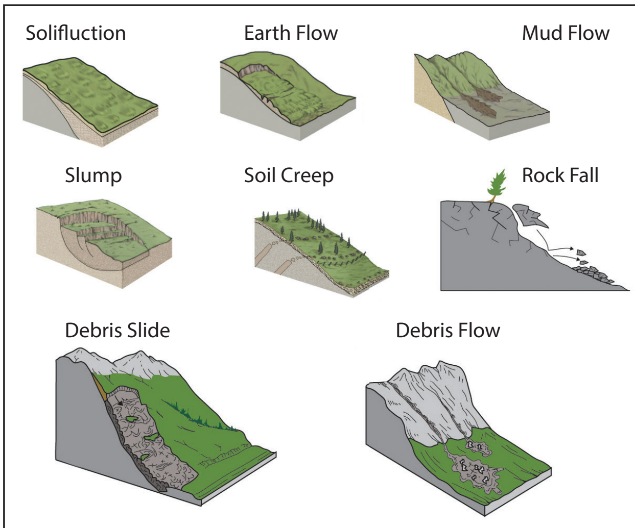
Figure 4.8 Mass Movement
