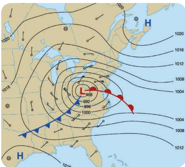
Figure 6.28 Cyclone
