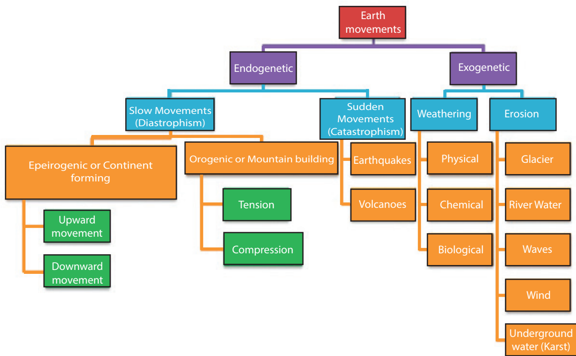
Figure 3.3 Earth's Forces
