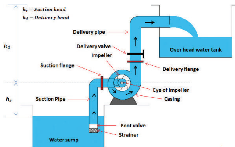
Centrifugal Pump
