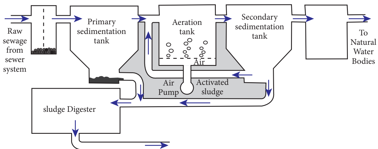
Secondary Sewage Treatment
