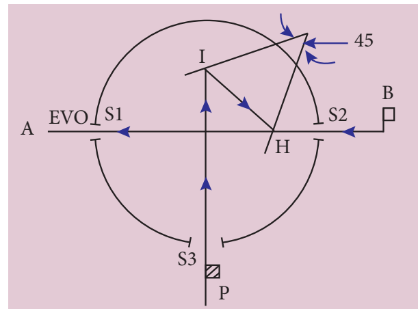
Optical Square
