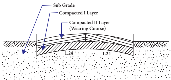
CROSS SECTION OF EARTH ROAD
