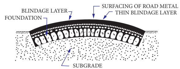
WATERBOUND MACADAM ROAD
