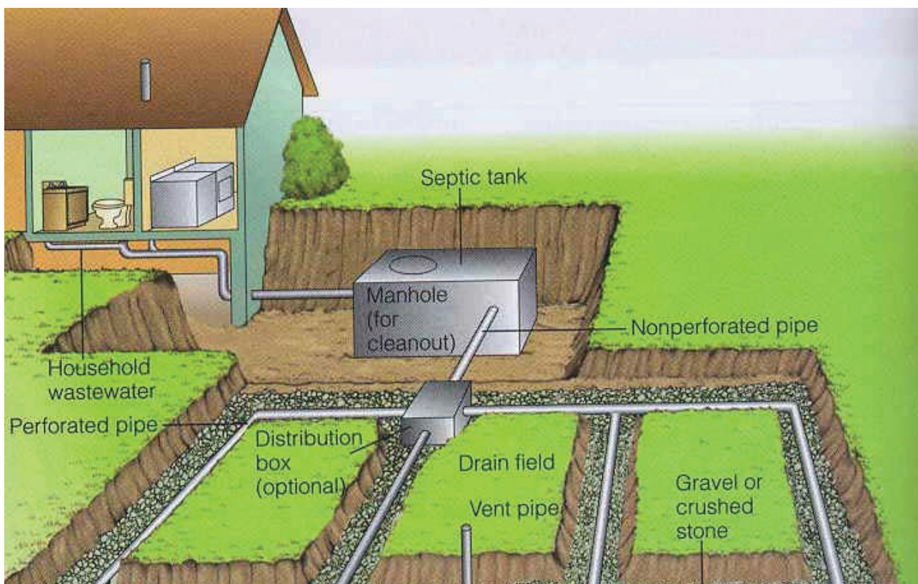
Flow Diagram of Sewage disposal
