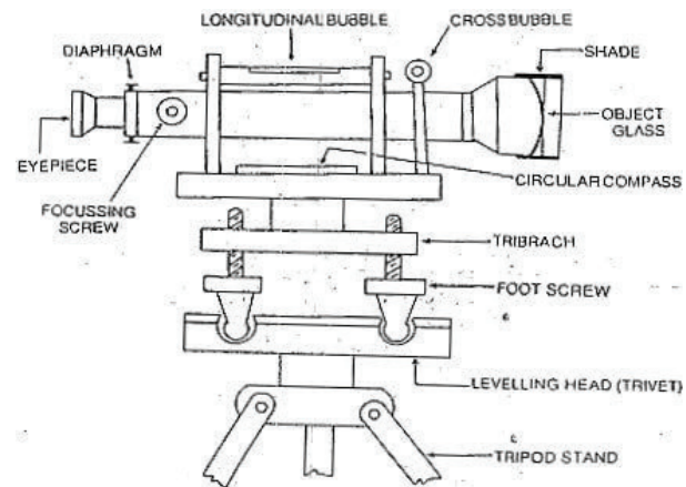
DUMPY LEVEL
