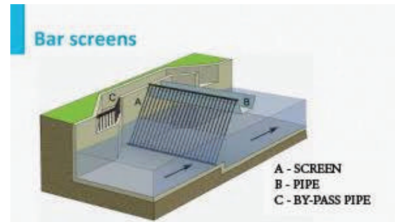
Bar screens
