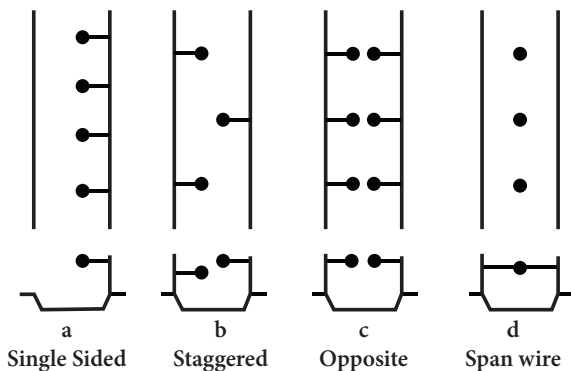
Lighting arrangement for 2 way Street
