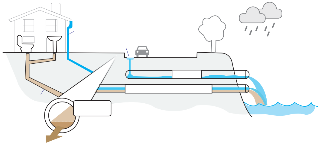
Partially Separated System
