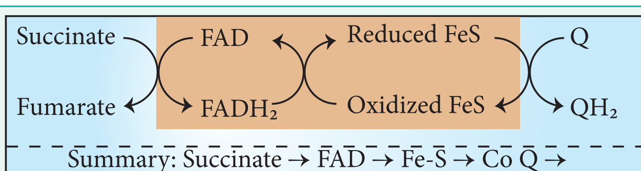
Figure 8.5 Reactions involved in complex II
