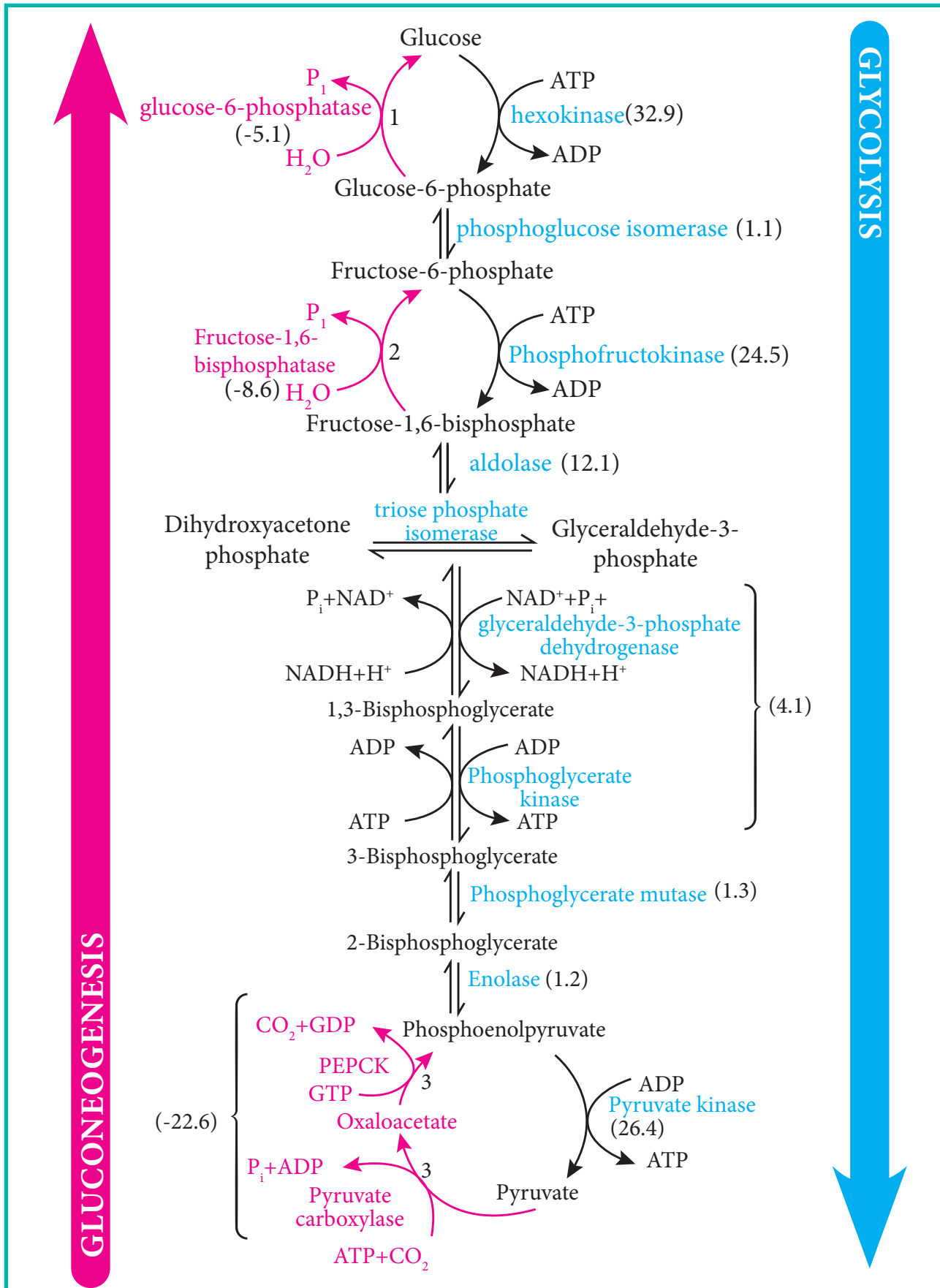
The \Delta G 's for the reactions in the direction of gluconeogenesis under physiological conditions in liver are given in parentheses in \text{kJ mol}^{-1} .
