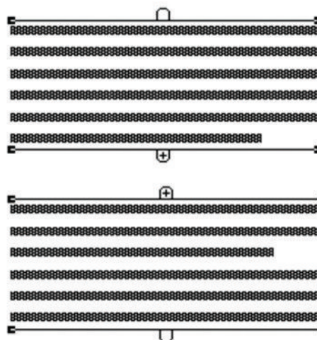
Figure 2.24 Threaded text-1
