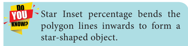
Figure 2.46 Polygon
