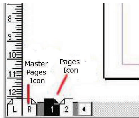
Figure 2.58 Master Pages
