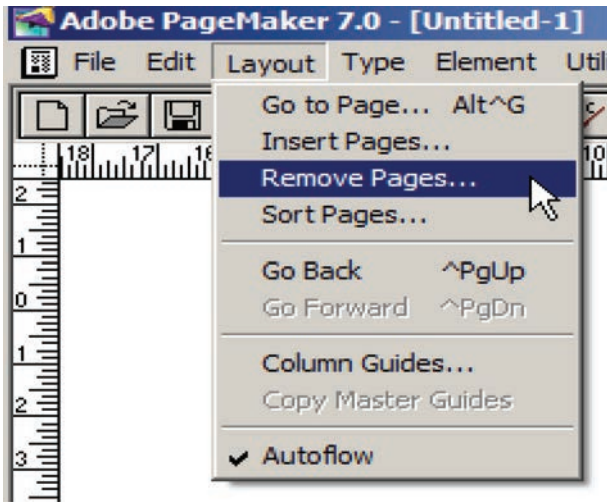
Figure 2.56 Remove pages
