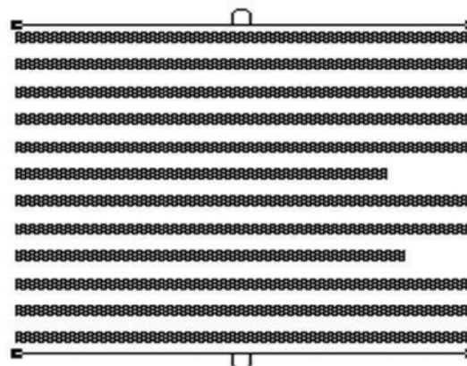
Figure 2.23 Unthreaded text
