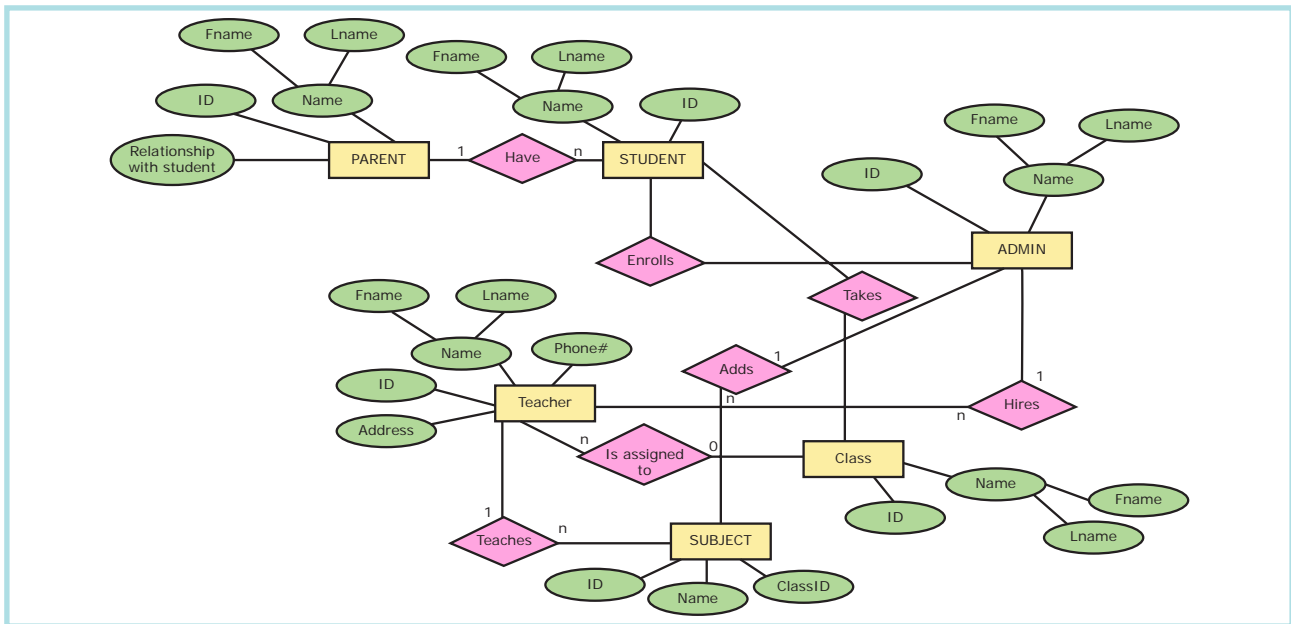
Figure: 3.12 ER-Diagram
