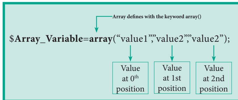
Figure 5.1 Indexed Arrays
