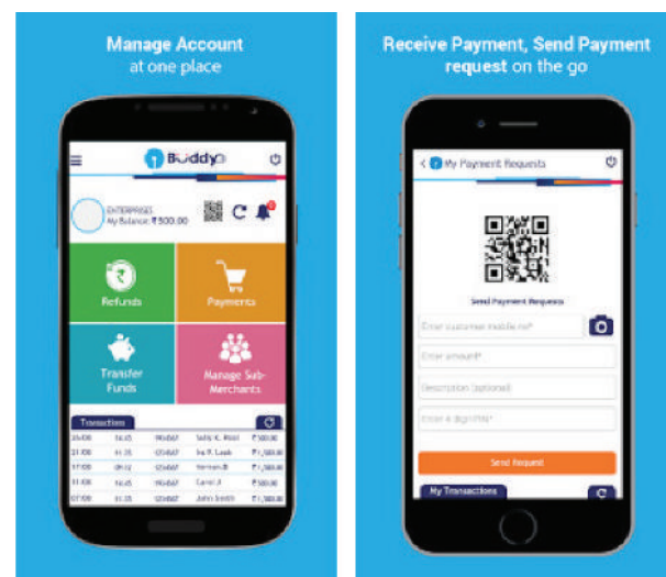
Figure 16.8 e-wallets
