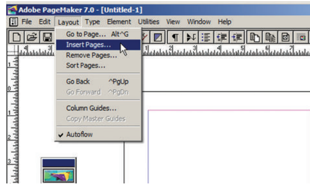
Figure 2.54 Insert Page
