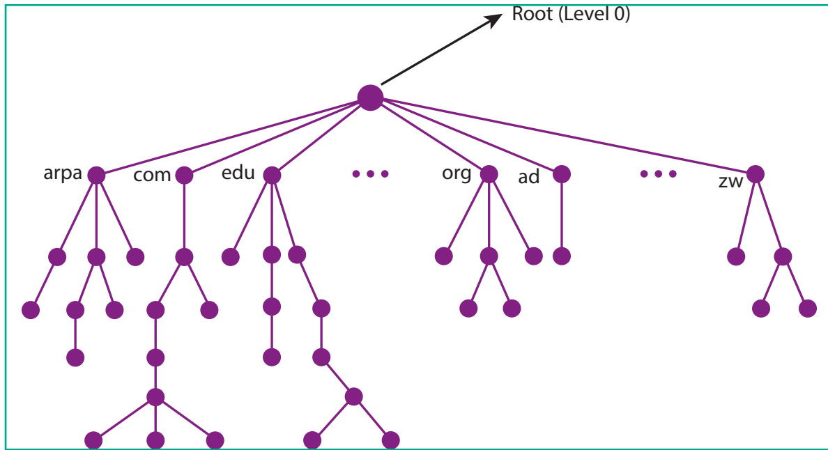
Figure 12.5 Domain Name Space
