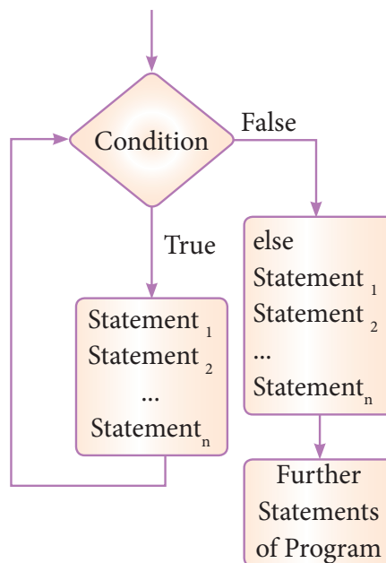
Fig 6.3 Diagram to illustrate how looping construct gets executed
