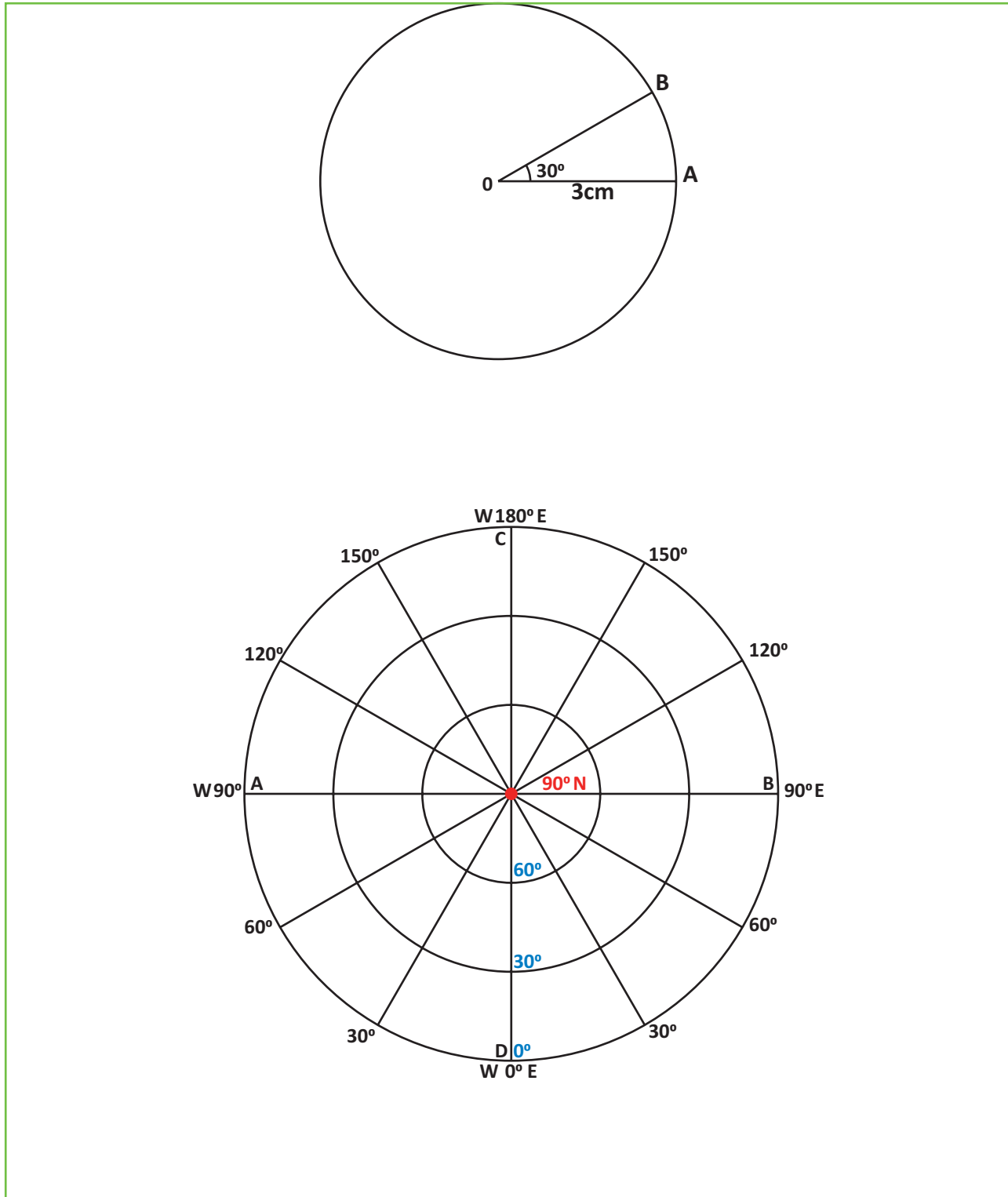
Polar Zenithal Equi distant projection
