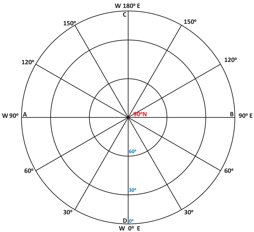
Polar Zenithal Equal area projection
