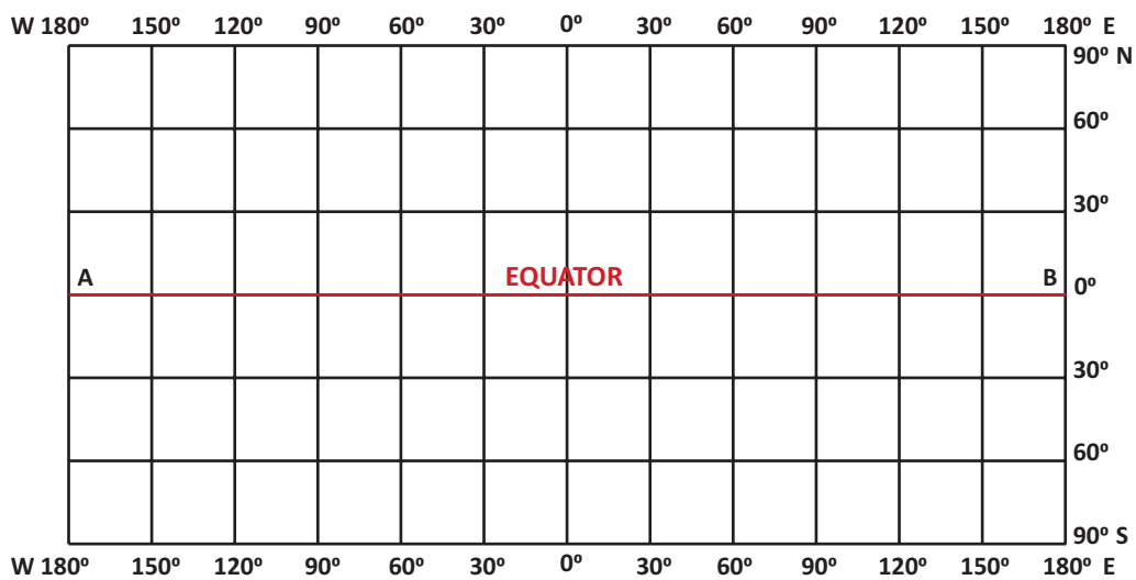
Cylindrical Equi-distant Projection
